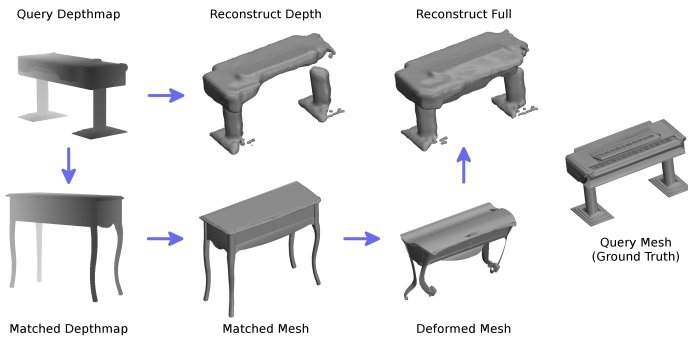
Figure 1: Pipeline for mesh reconstruction from depth image. A depth image of an piano is matched to a depth image of a table. The exemplar table is retrieved and deformed to better fit the observed depth points. Finally, a reconstructed mesh is created based on the observed depth points and deformed table exemplar. This mesh outperforms a mesh constructed from only depth points alone (“Reconstruct Depth”).
